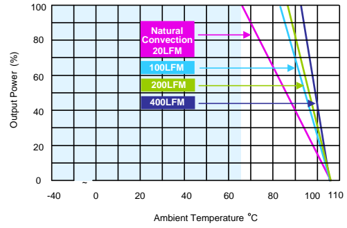
MKWI40-24S24,MKWI40-48S24 Derating Curve with Heatsink
