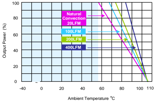
MKWI40-24S24,MKWI40-48S24 Derating Curve without Heatsink
