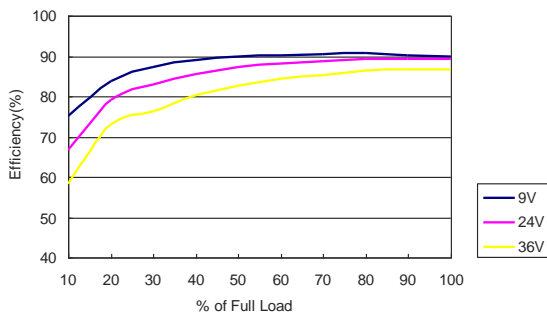
MKW140-24S24 Efficiency vs Load Current
